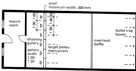
2 Shooting range for air and CO 2 guns: covered shooting gallery, range in the open
